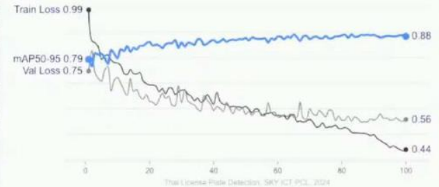
License Plate Detection Training Results
